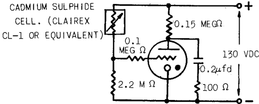
740I ACTING AS A RELAY FOR A CADMIUM SULPHIDE PHOTO CELL
