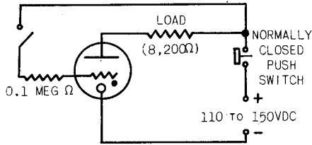
740I USED AS A MECHANICALLY OPERATED RELAY
