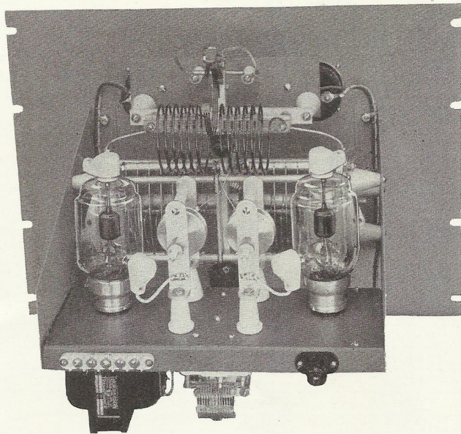
Top View TW-75 AMPLIFIER
