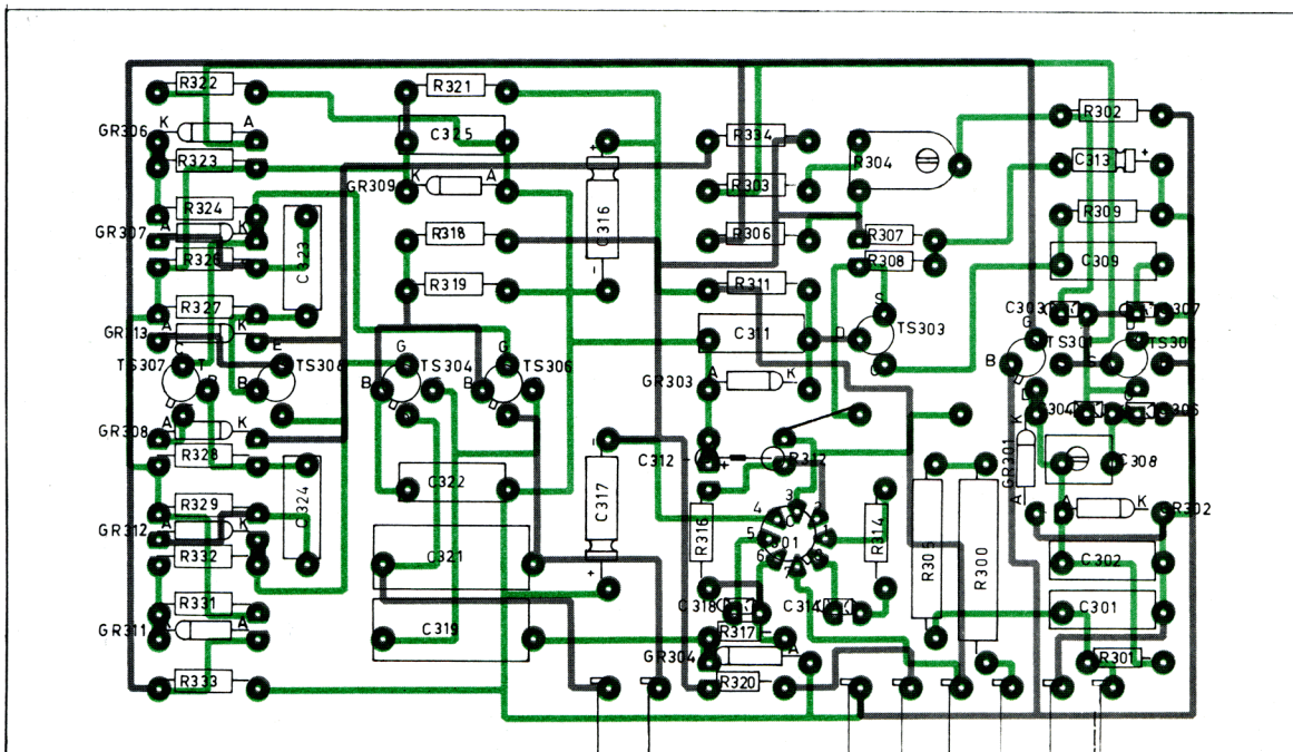
Fig. 23. Printed circuit Unit 12 (Chopper amplifier)
