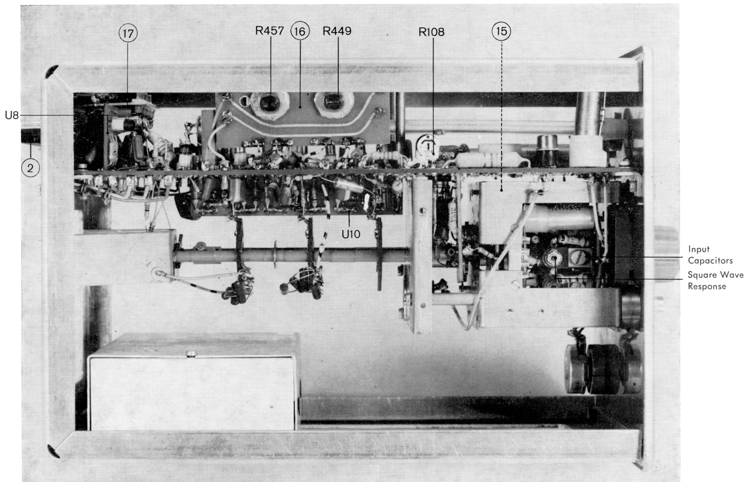
Fig. 14. Left-hand view
