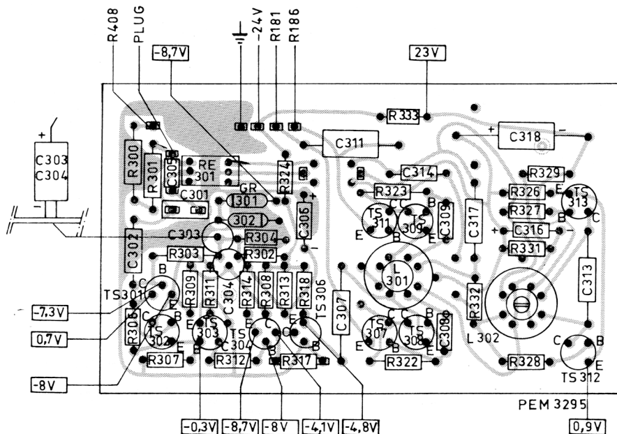
Fig. 22. Printed circuit U 12 (Chopper Amplifier)
