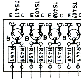
Fig. 20. Printed circuit Unit 8 (Final stage)
