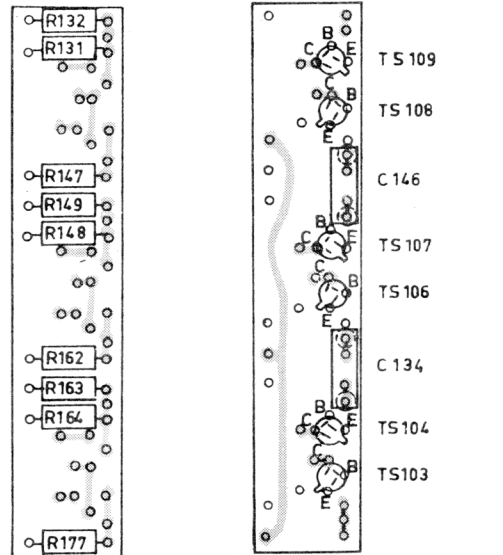
Fig. 20. Printed circuit U 10 (H.F. amplifier)
