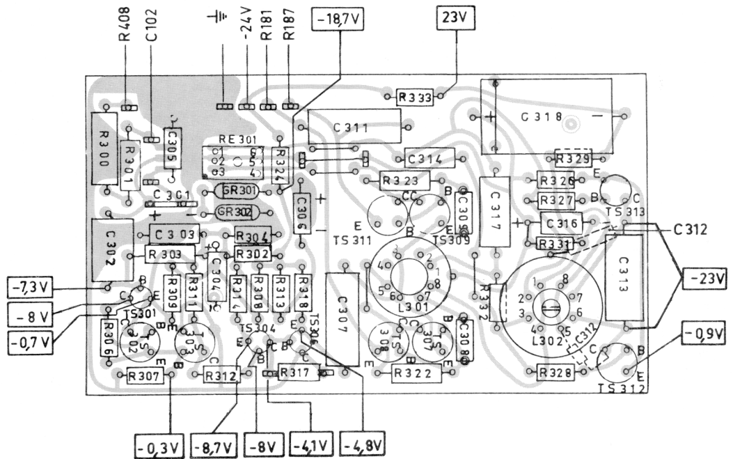
Fig. 22. Printed circuit U 12 (Chopper Amplifier)
