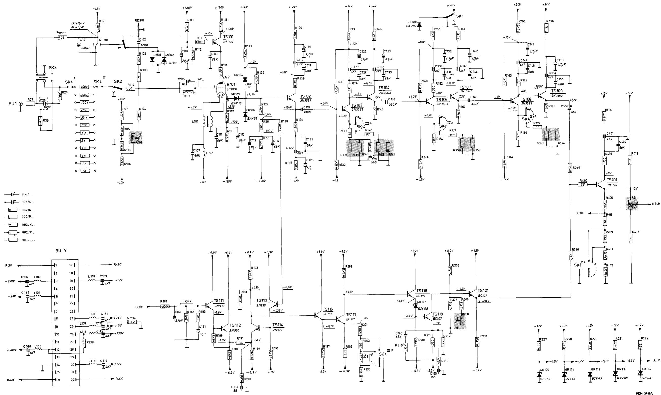
Fig. 26. HF and LF amplifier circuit
