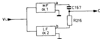
Fig. 12. Operation of the crossover filter
